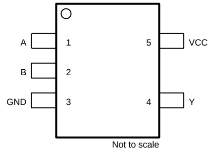
Figure 5-1. SN74AHC1G02-Q1 DBV Package, 5-Pin SOT-23; DCK Package, 5-Pin SC-70 (Top View)
