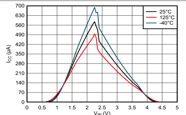
Figure 6-2. Supply Current Across Input Voltage, 5-V Supply
