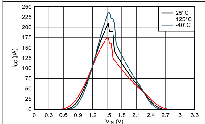
Figure 6-3. Supply Current Across Input Voltage, 3.3-V Supply
