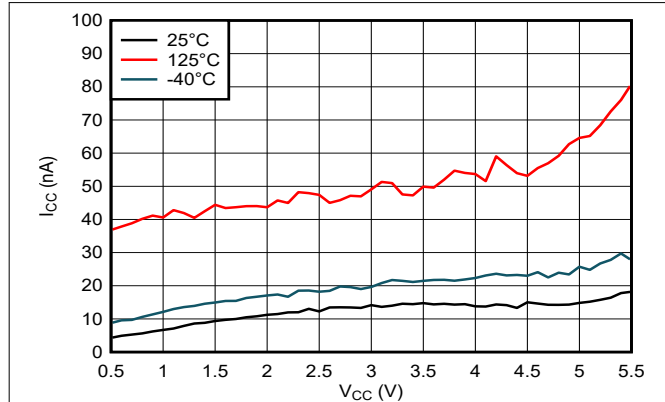
Figure 6-1. Supply Current Across Operating Voltage
