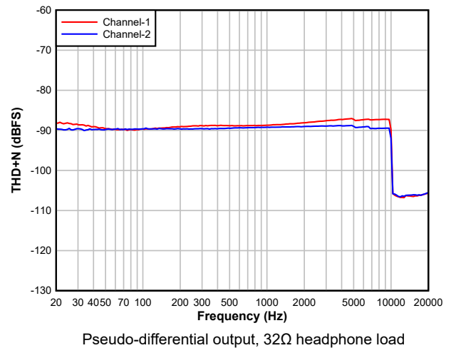
Figure 5-9. DAC THD+N Level vs Frequency
