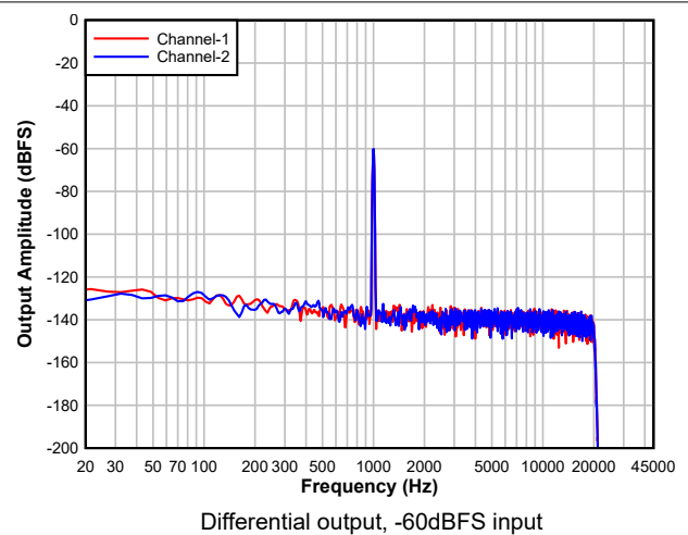
Figure 5-11. DAC FFT
