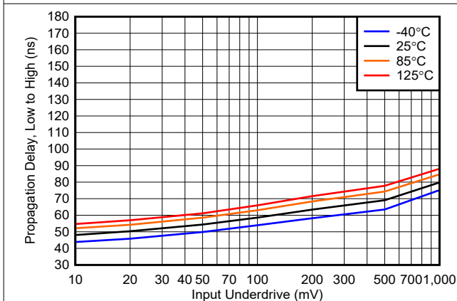
Figure 6-29. Propagation Delay, (Low to High) vs. Input Underdrive, 40V
