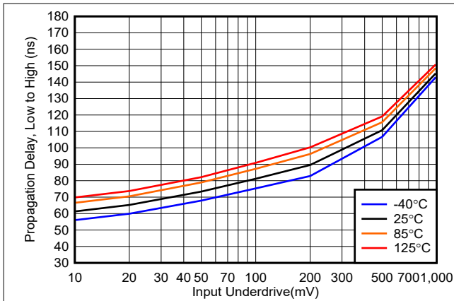
Figure 6-25. Propagation Delay, (Low to High) vs. Input Underdrive, 3.3V
