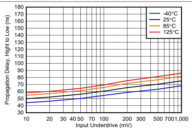
Figure 6-30. Propagation Delay, (High to Low) vs. Input Underdrive, 40V
