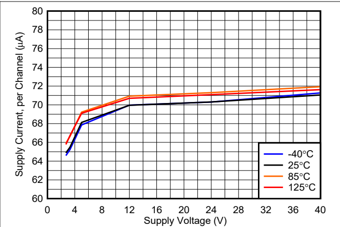
Figure 6-14. Supply Current vs. Supply Voltage, Output High, No Load
