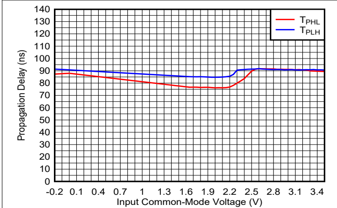
Figure 6-15. Propagation Delay vs. Common-Mode, 3.3V
