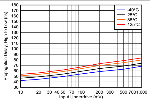
Figure 6-28. Propagation Delay, (High to Low) vs. Input Underdrive, 12V
