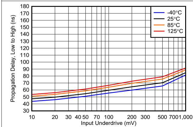
Figure 6-27. Propagation Delay, (Low to High) vs. Input Underdrive, 12V
