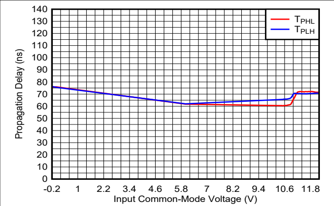
Figure 6-16. Propagation Delay vs. Common-Mode, 12V
