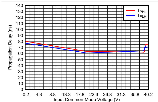
Figure 6-17. Propagation Delay vs. Common-Mode, 40V
