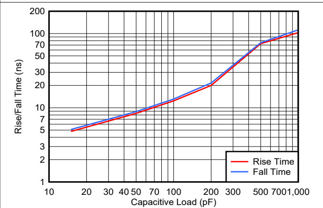
Figure 6-18. Rise/Fall Time vs. Capacitive Load, 12V
