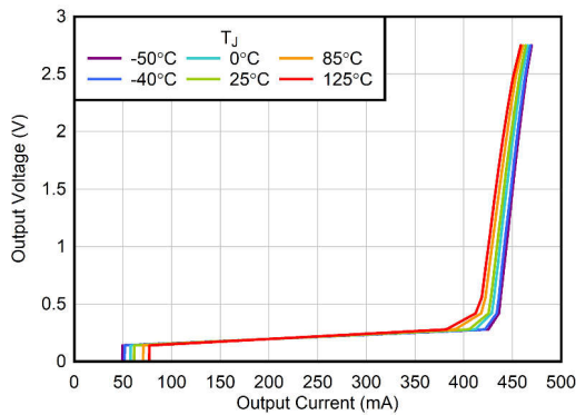
Figure 5-9. Current Limit
