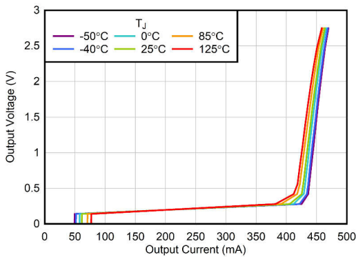
Figure 5-9. Current Limit
