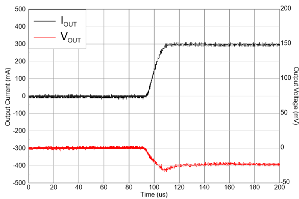
Figure 5-9. Current Limit
