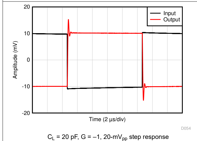
Figure 6-35. Small-Signal Step Response
