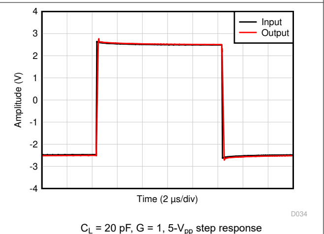
Figure 6-36. Large-Signal Step Response
