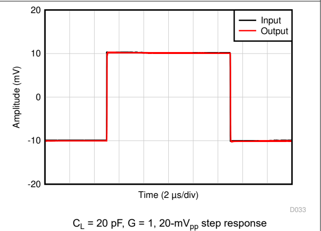
Figure 6-34. Small-Signal Step Response
