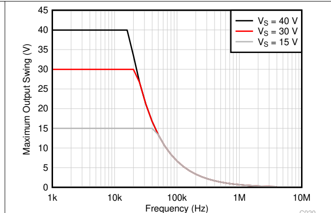
Figure 6-38. Maximum Output Voltage vs Frequency
