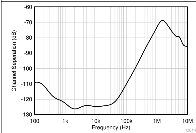
Figure 6-39. Channel Separation vs Frequency
