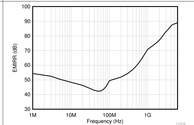
Figure 6-40. EMIRR (Electromagnetic Interference Rejection Ratio) vs Frequency
