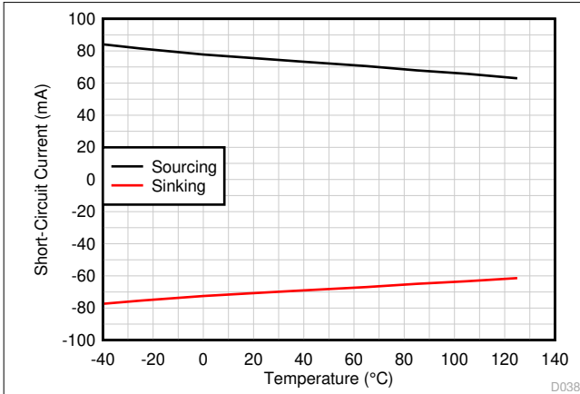
Figure 6-37. Short-Circuit Current vs Temperature
