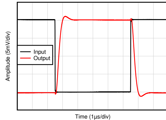
C_L = 20\text{ pF} , G = 1 , 20-mV step response Figure 6-34. Small-Signal Step Response, Falling
