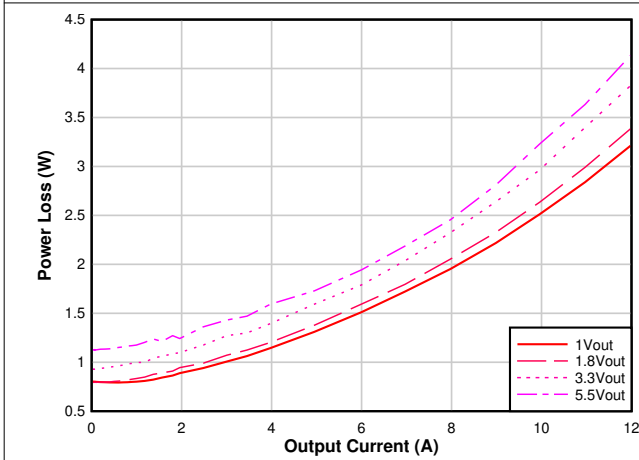
Figure 6-5. Power Dissipation vs Output Current, V_{IN} = 12 V, F_{SW} = 1 MHz
