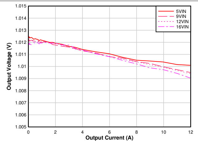
Figure 6-6. Output Voltage Regulation vs Output Current, V_{OUT} = 1.0 V, F_{SW} = 1 MHz
