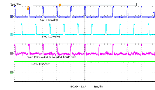
Figure 8-46. Output Ripple – 12-A Load
