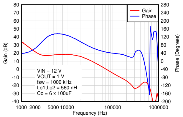
Figure 8-37. Bode Plot
