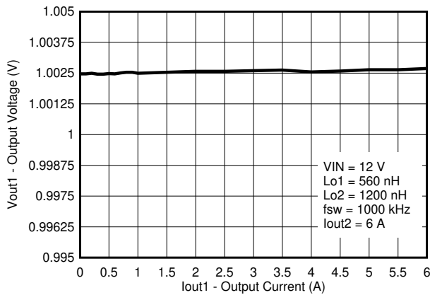
Figure 8-5. V_{OUT1} Load Regulation
