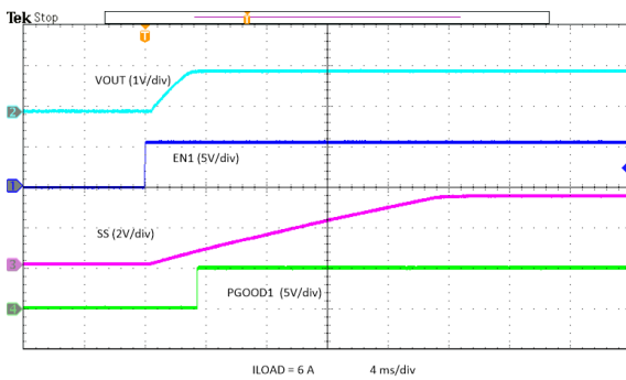
Figure 8-39. Power Up with EN
