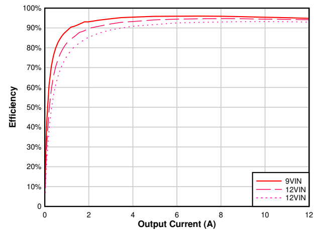
Figure 6-4. Efficiency vs Output Current, V_{OUT} = 5.5 V, F_{SW} = 1 MHz
