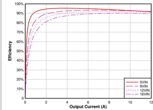
Figure 6-3. Efficiency vs Output Current, V_{OUT} = 3.3 V, F_{SW} = 1 MHz
