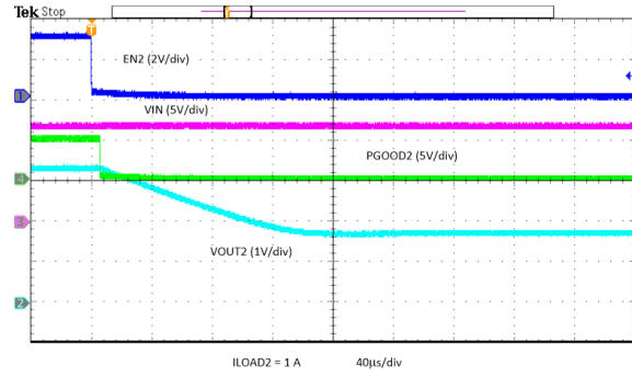
Figure 8-22. Power Down with EN 2 with Pre Bias
