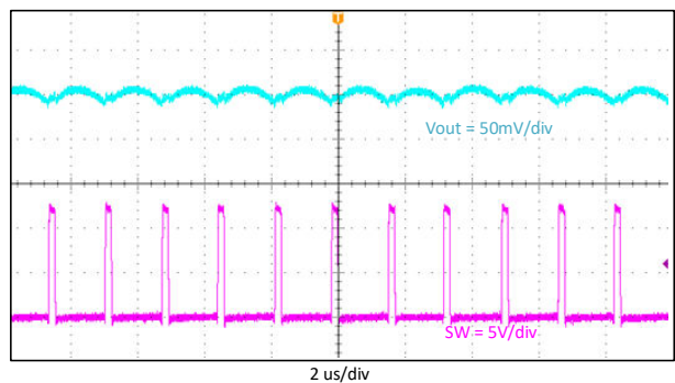
Figure 8-7. Output Voltage Ripple, I_{out} = 3 A
