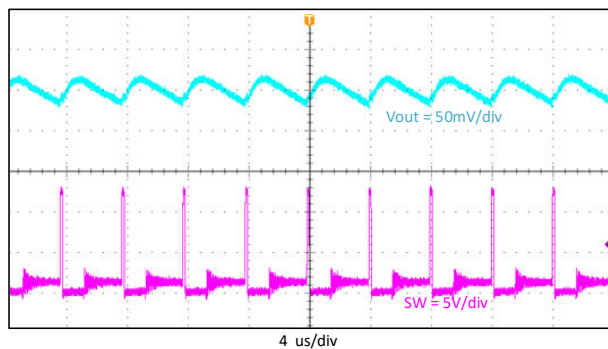
Figure 8-6. Output Voltage Ripple, I_{out} = 0.3 A
