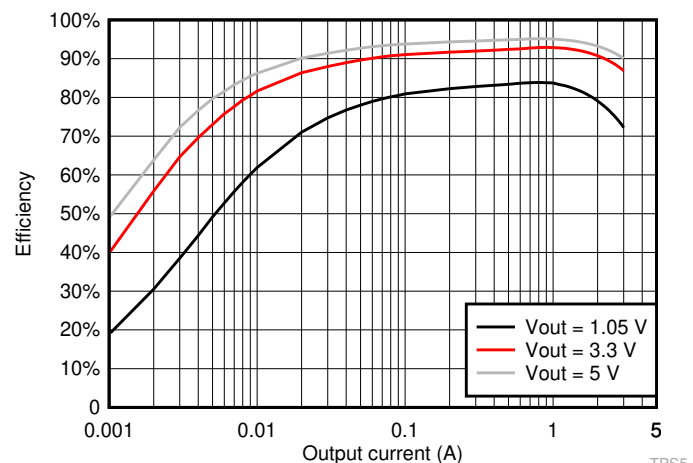
TPS563202 Efficiency
