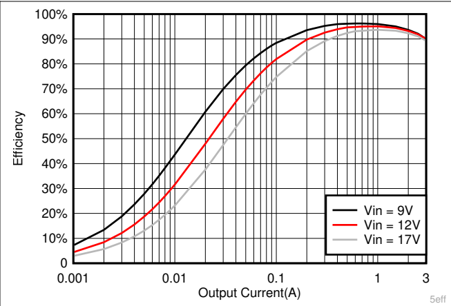
Figure 7-14. V_{OUT} = 5\text{-V} Efficiency, L = 4.7\ \mu\text{H}
