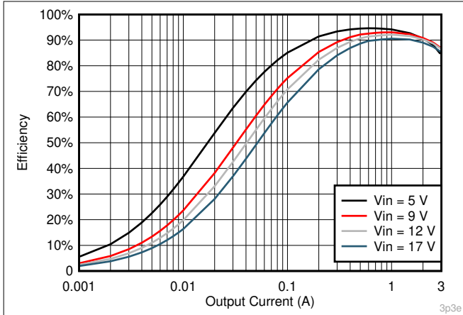
Figure 7-13. V_{OUT} = 3.3\text{-V} Efficiency, L = 3.3\ \mu\text{H}
