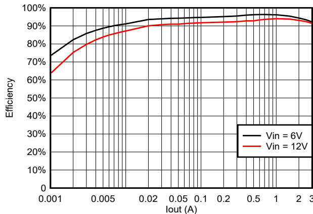
Figure 6-15. TPS563252 Efficiency at 3.3 V_{OUT} with a 2.2- \mu\text{H} Inductor
