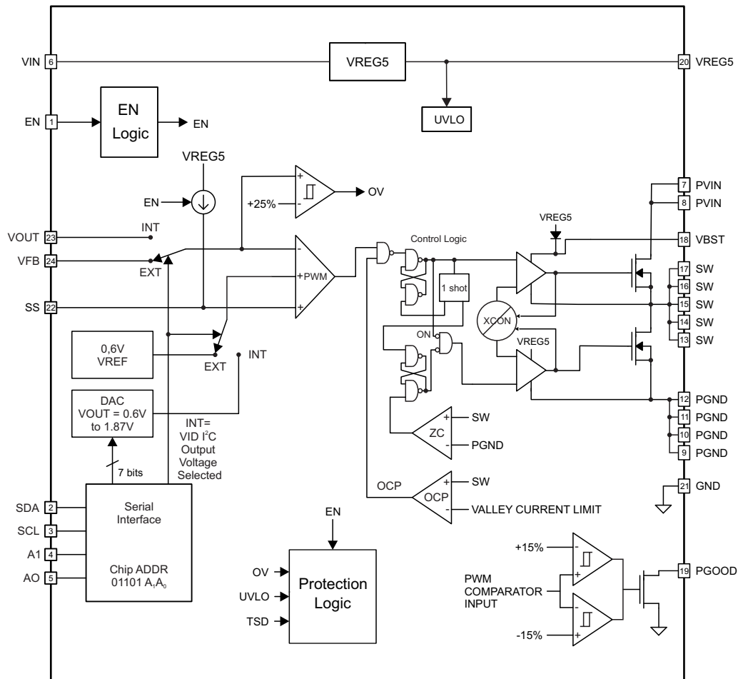
Figure 28. TPS56C20 24 Terminal
