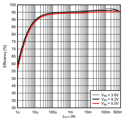
Figure 8-6. Efficiency at V_{OUT} = 3.3V
