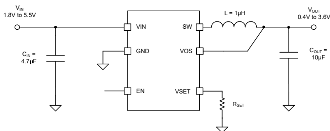
Typical Application
