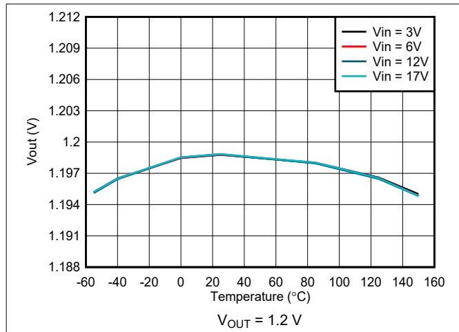
Figure 7-7. Output Voltage Accuracy – VSET Selected
