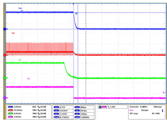
Figure 9-65. Shutdown Timing with Output Discharge Enabled
