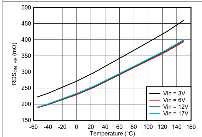
Figure 7-11. High-Side R_{DS(on)} vs Temperature
