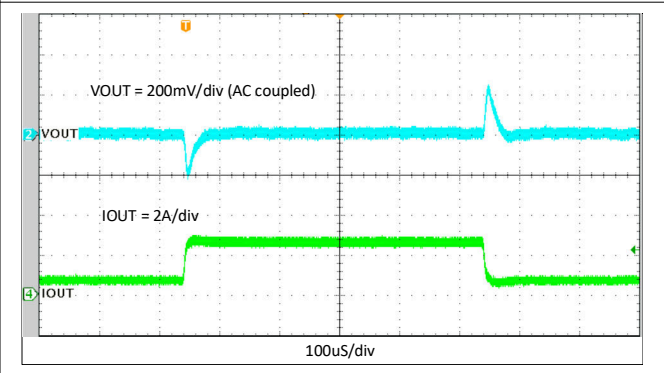
Figure 10-19. Load Transient Response, 0.5 to 2.5 A, Slew Rate = 0.8 A/ \mu S
