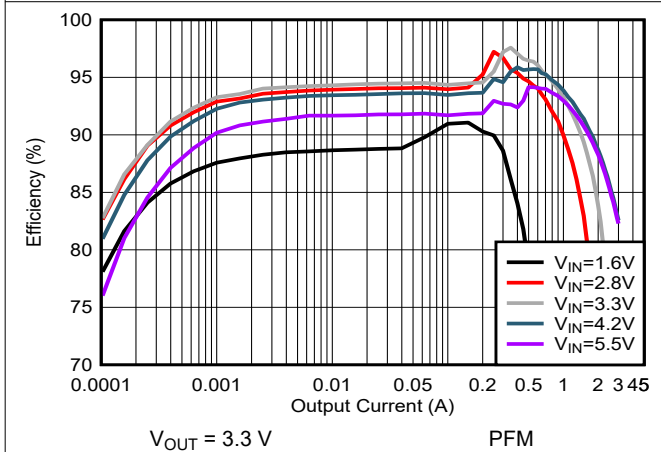
Figure 9-4. Efficiency vs Input Voltage (PFM)
