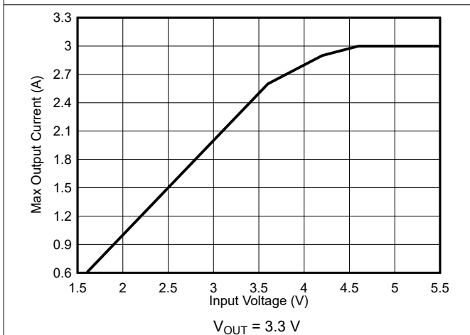
Figure 9-6. Typical Output Current Capability vs Input Voltage
