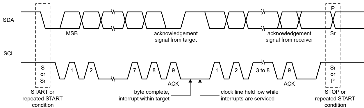
Figure 8-7. Bus Protocol
