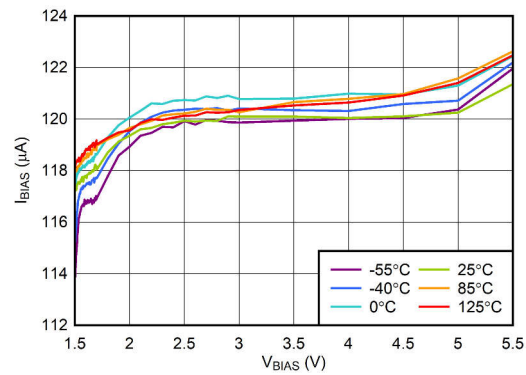
Figure 6-6. V_{\text{BIAS}} Input Current vs V_{\text{BIAS}}
