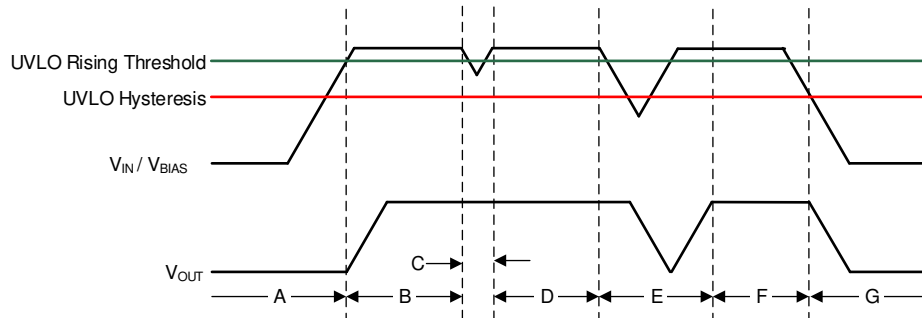
Figure 8-2. Typical V_{IN} or V_{BIAS} UVLO Circuit Operation
