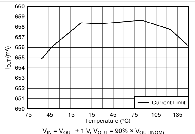
Figure 6-26. Output Current Limit vs Temperature
