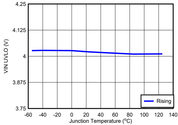
Figure 6-7. V IN UVLO
