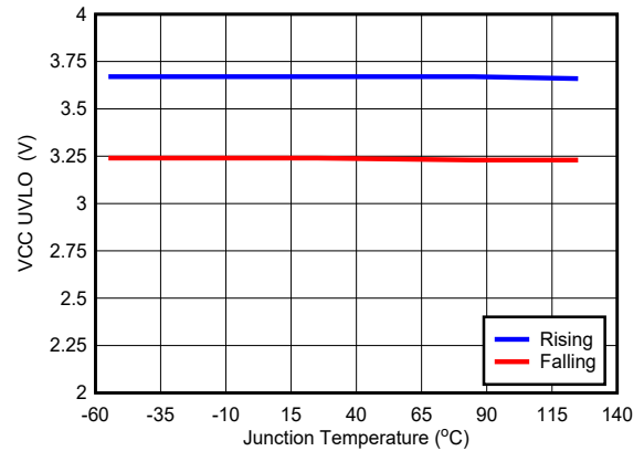
Figure 6-8. V CC UVLO
