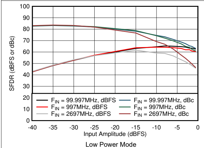
Figure 5-59. SFDR vs Input Amplitude in Low Power Mode
