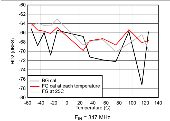
Figure 5-45. HD2 vs Temperature
