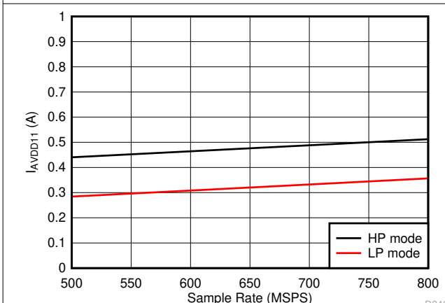
Figure 5-79. Quad Channel, I_{VA11} vs F_S Independent of JMODE
