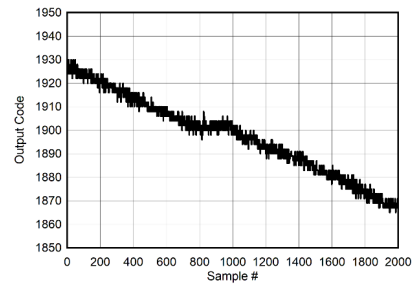
BG Calibration, midscale input voltage, ADC_SRC_DLY=31, MUX_DLY=30
