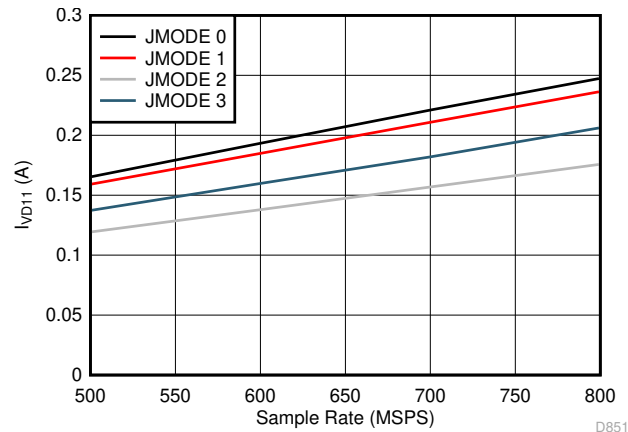
Figure 5-94. Dual Channel, I_{VD11} vs F_S for JMODES 0 - 3
