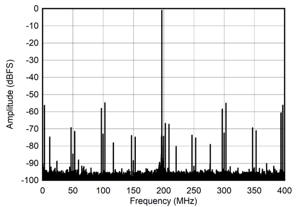
PLL on, suppression off Figure 5-16. Single Tone FFT at 997 MHz and -1dBFS
