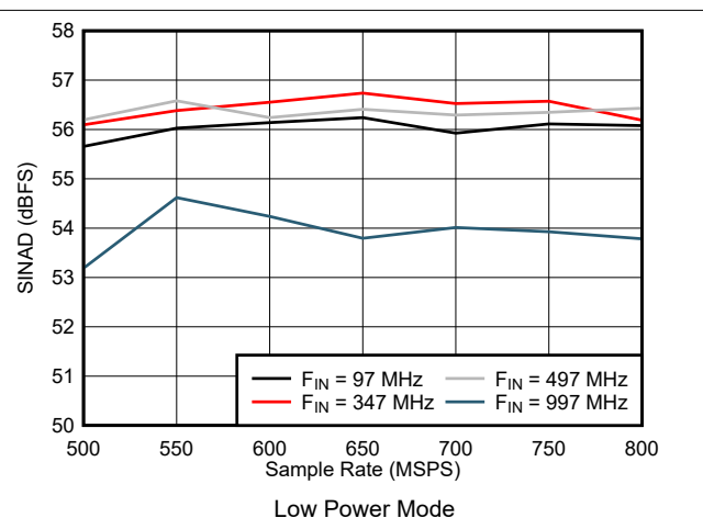
Figure 5-56. SINAD vs Sample Rate in Low Power Mode
