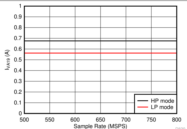
Figure 5-78. Quad Channel, I_{VA19} vs F_S Independent of JMODE
