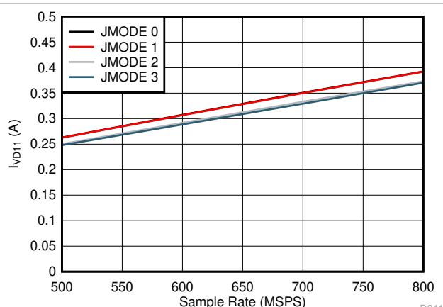
Figure 5-80. Quad Channel, I_{VD11} vs F_S for JMODES 0 - 3 Independent of Power Mode
