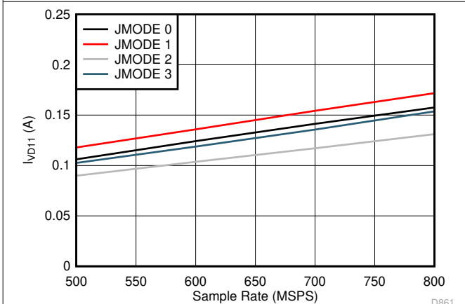
Figure 5-107. Single Channel, I_{VD11} vs F_S for JMODES 0 - 3
