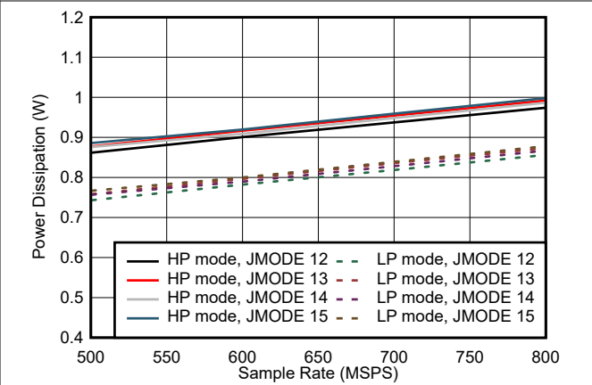
Figure 5-104. Single Channel, Power Dissipation vs F_S for JMODES 12 - 15
