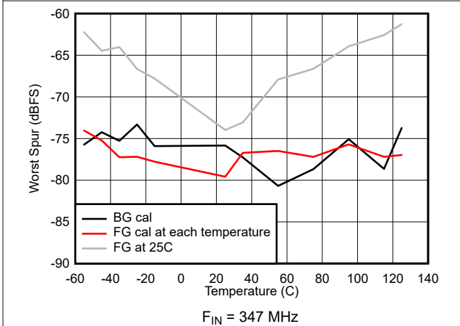
Figure 5-47. worst non-HD spur vs Temperature
