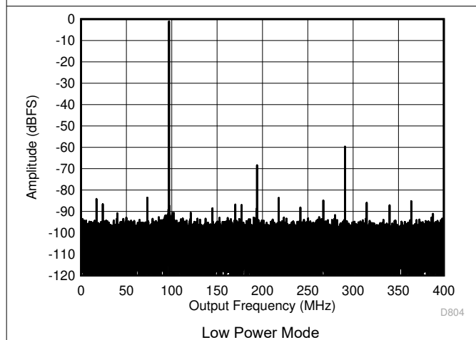
Figure 5-11. Single Tone FFT at 897 MHz and -1dBFS
