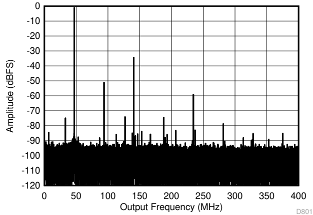
Low Power Mode Figure 5-13. Single Tone FFT at 3247 MHz and -1dBFS
