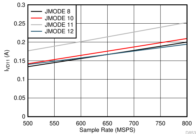
Figure 5-96. Dual Channel, I_{VD11} vs F_S for JMODES 8 - 12
