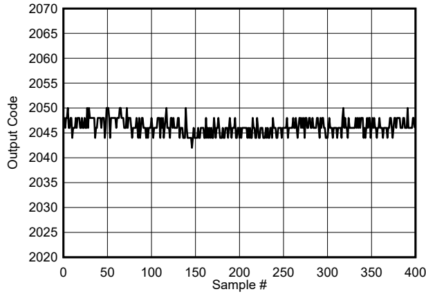
BG Calibration, midscale input voltage, ADC_SRC_DLY=31, MUX_DLY=30
