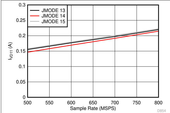
Figure 5-97. Dual Channel, I_{VD11} vs F_S for JMODES 13 - 15
