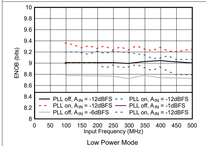
Figure 5-53. ENOB vs Input Frequency in Low Power Mode
