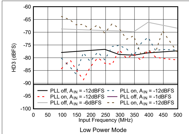
Figure 5-51. HD3 vs Input Frequency in Low Power Mode
