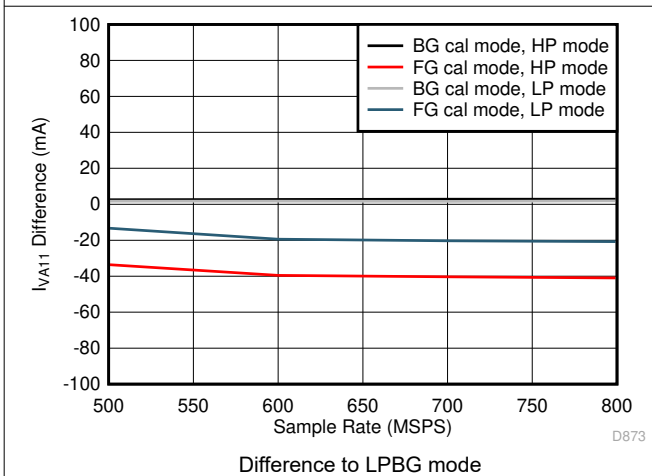
Figure 5-113. Single Channel, I_{VA11} vs F_S over Modes
