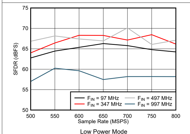
Figure 5-55. SFDR vs Sample Rate in Low Power Mode
