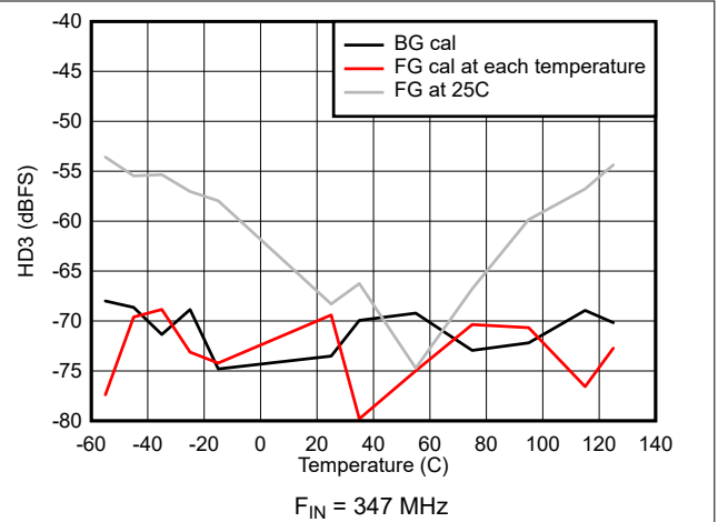
Figure 5-46. HD3 vs Temperature
