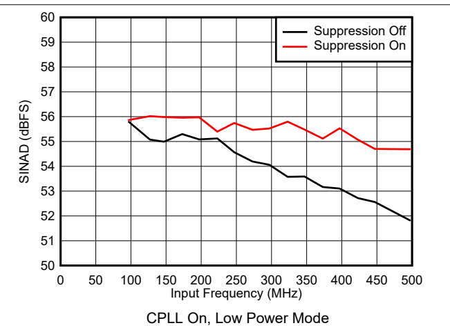
Figure 5-62. SINAD vs Input Frequency
