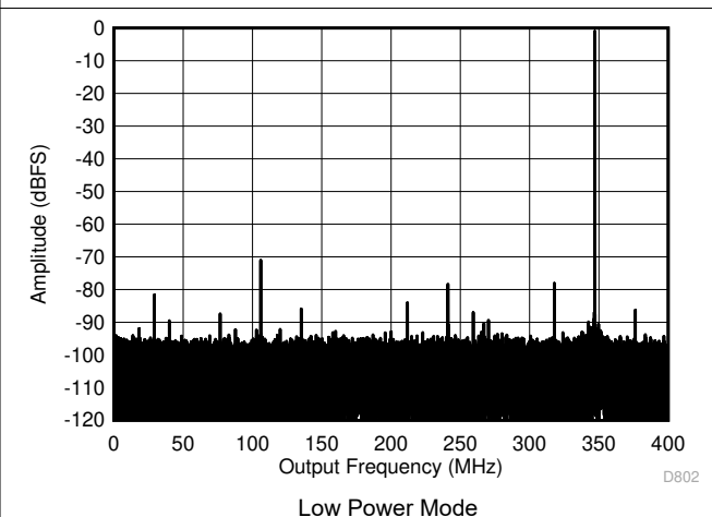
Figure 5-10. Single Tone FFT at 347 MHz and -1dBFS
