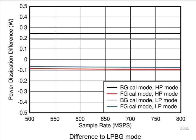
Figure 5-84. Quad Channel, Power Dissipation vs F_S over Modes
