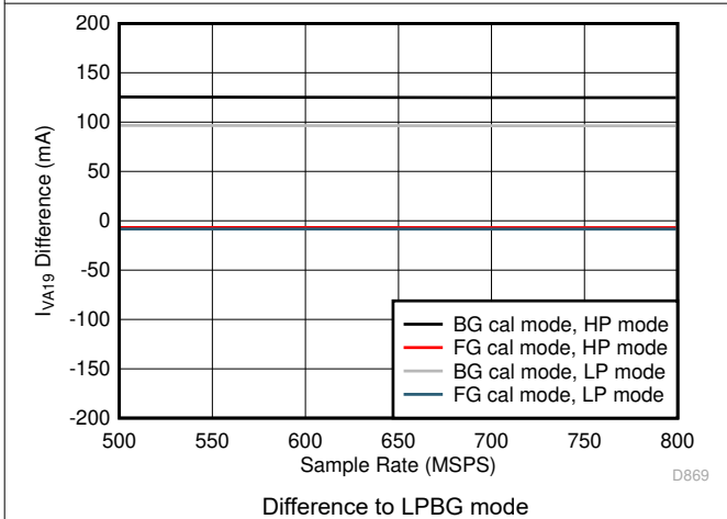
Figure 5-99. Dual Channel, I_{VA19} vs F_S over Modes
