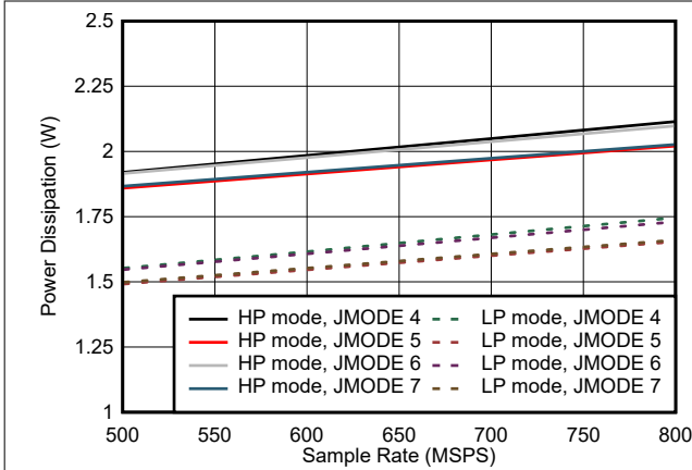
Figure 5-75. Quad Channel, Power Dissipation vs F_S for JMODES 4 - 7
