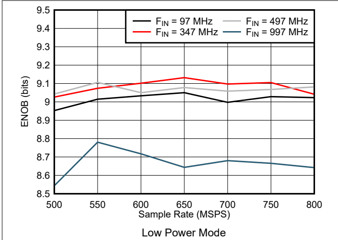
Figure 5-57. ENOB vs Sample Rate in Low Power Mode
