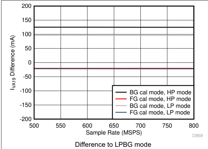
Figure 5-85. Quad Channel, I_{VA19} vs F_S over Modes
