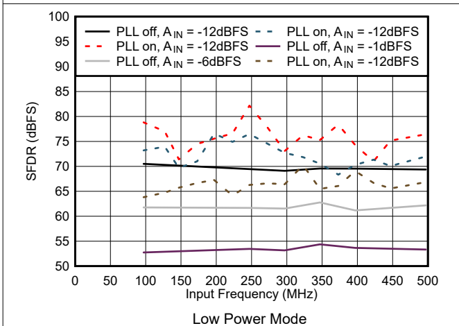
Figure 5-49. SFDR vs Input Frequency in Low Power Mode
