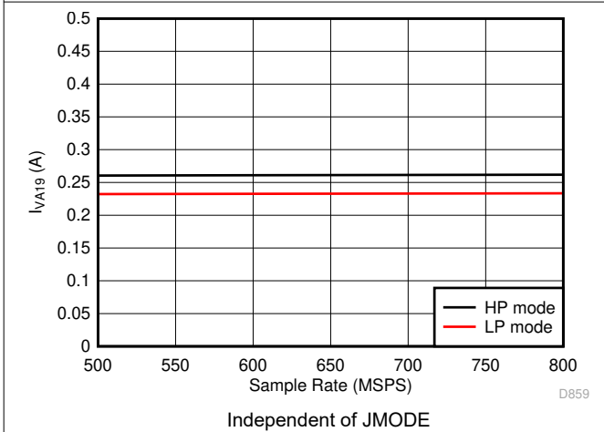
Figure 5-105. Single Channel, I_{VA19} vs F_S
