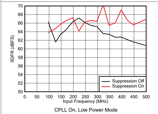
Figure 5-61. SFDR vs Input Frequency
