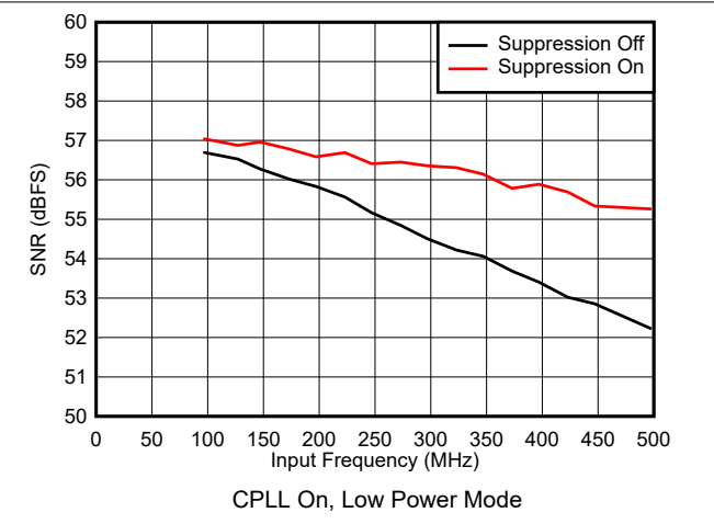
Figure 5-60. SNR vs Input Frequency
