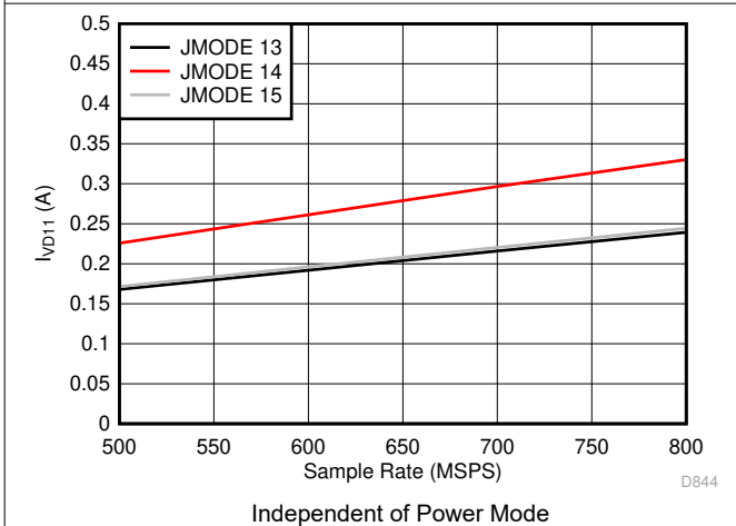
Figure 5-83. Quad Channel, I_{VD11} vs F_S for JMODES 13-15
