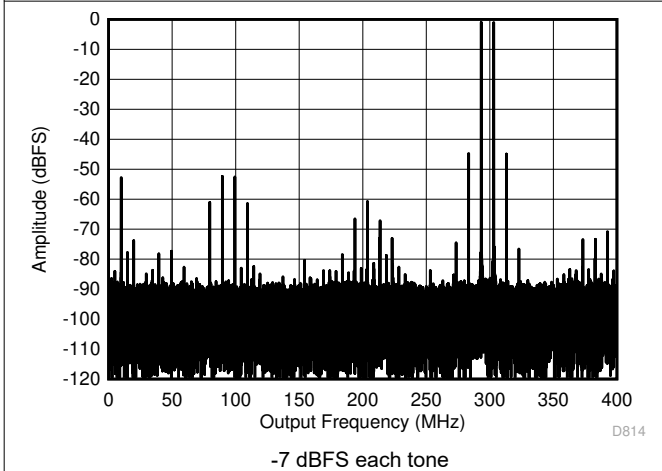
Figure 5-71. Two Tone FFT at 3498 MHz in Low Power Mode
