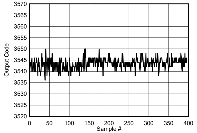
BG Calibration, midscale input voltage, ADC_SRC_DLY=31, MUX_DLY=30
