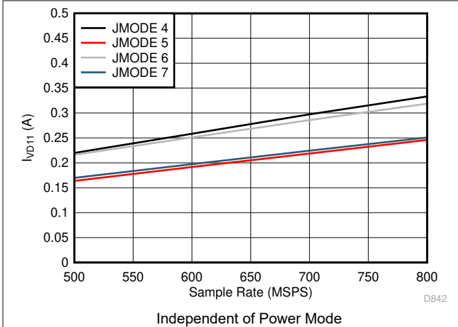
Figure 5-81. Quad Channel, I_{VD11} vs F_S for JMODES 4 - 7
