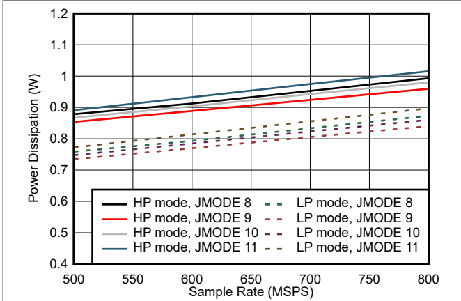
Figure 5-103. Single Channel, Power Dissipation vs F_S for JMODES 8 - 11
