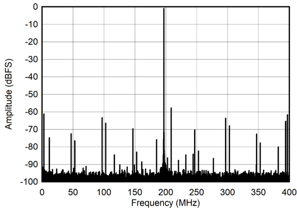
Low Lower Mode, PLL on, suppression on
