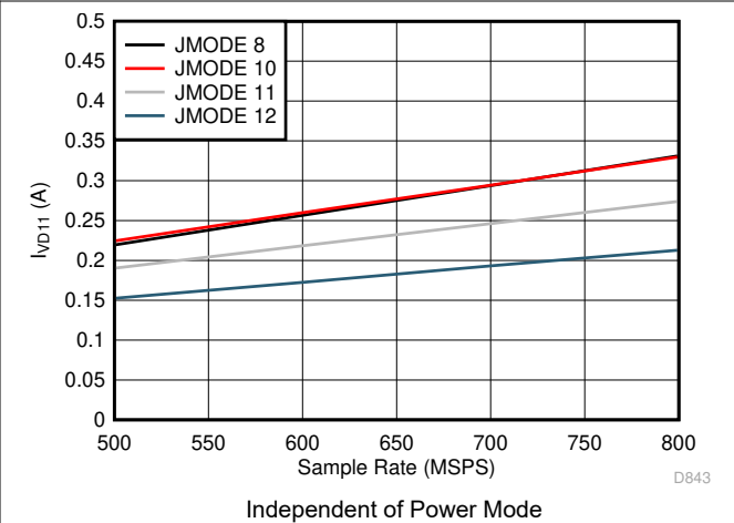
Figure 5-82. Quad Channel, I_{VD11} vs F_S for JMODES 8-12
