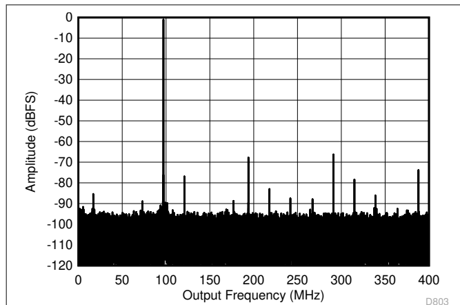
Figure 5-7. Single Tone FFT at 897 MHz and -1dBFS
