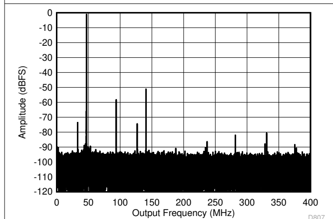
Figure 5-9. Single Tone FFT at 3247 MHz and -1dBFS
