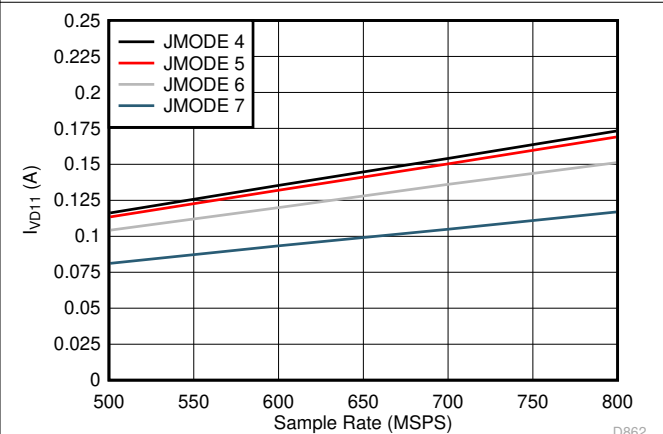
Figure 5-108. Single Channel, I_{VD11} vs F_S for JMODES 4 - 7
