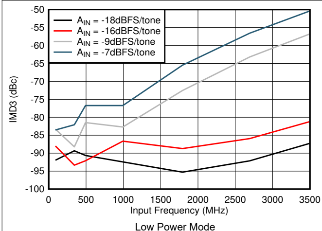
Figure 5-73. IMD3 vs Input Frequency in Low Power Mode
