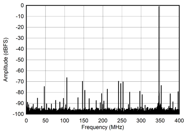
PLL on, suppression on Figure 5-15. Single Tone FFT at 347 MHz and -1dBFS
