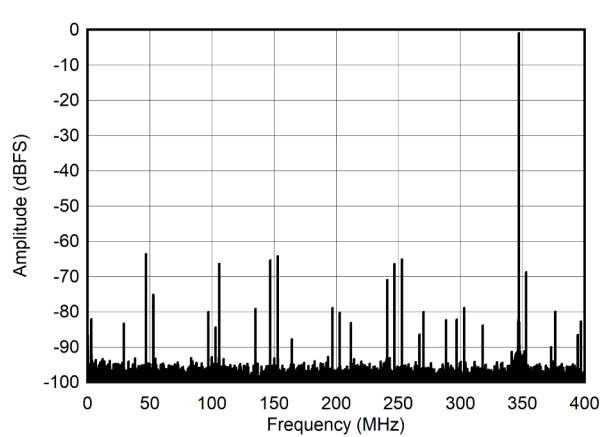
PLL on, suppression off Figure 5-14. Single Tone FFT at 347 MHz and -1dBFS
