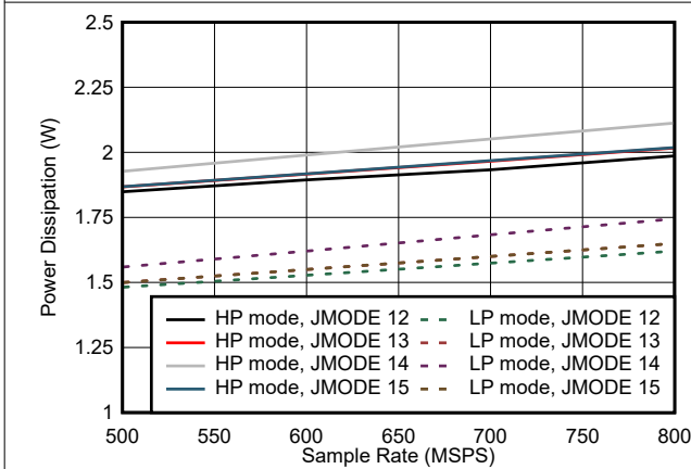
Figure 5-77. Quad Channel, Power Dissipation vs F_S for JMODES 12 - 15
