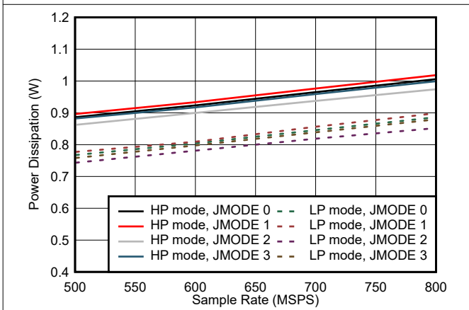
Figure 5-101. Dual Channel, Power Dissipation vs F_S for JMODES 0 - 3
