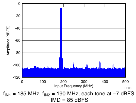
Figure 10. FFT for Two-Tone Input Signal (-7 dBFS)
