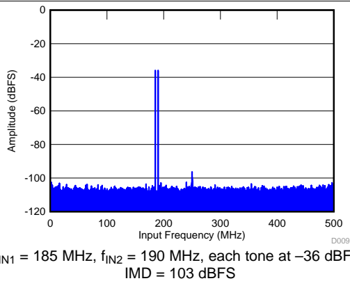
Figure 11. FFT for Two-Tone Input Signal (-36 dBFS)
