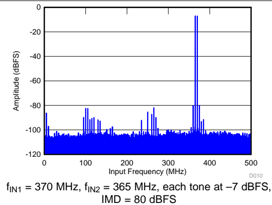
Figure 12. FFT for Two-Tone Input Signal (-7 dBFS)
