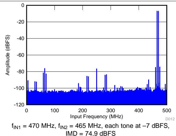
Figure 14. FFT for Two-Tone Input Signal (-7 dBFS)
