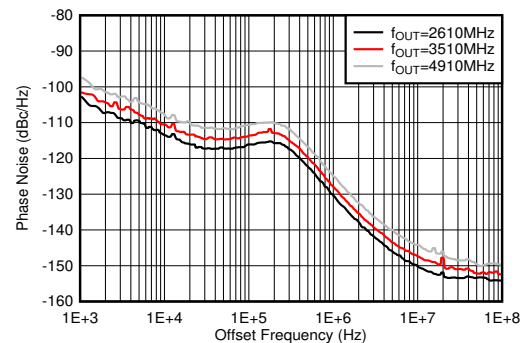
Figure 5-583. Phase Noise for 10-GHz VCO vs Offset Frequency and f_{OUT} at 25°C
