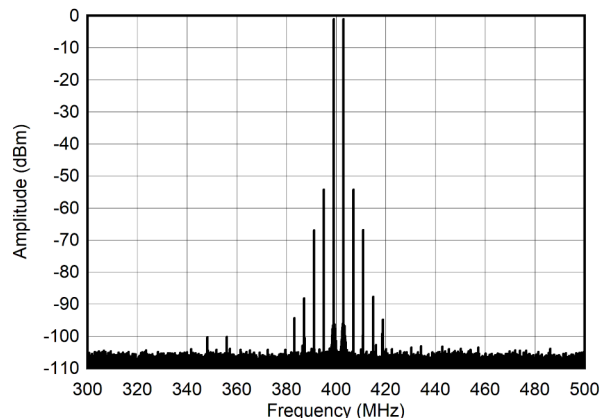
Figure 5-259. Dual Tone Spectrum at 400 MHz and -7 dBFS ( \pm 100\text{MHz} )
