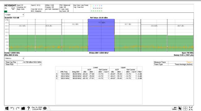
Figure 5-504. TX 100-MHz NR Output Spectrum at 4.9 GHz
