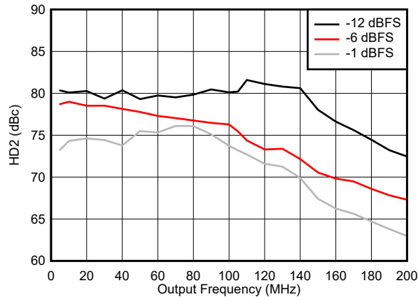
Figure 5-236. HD2 vs Frequency 0 - 200 MHz
