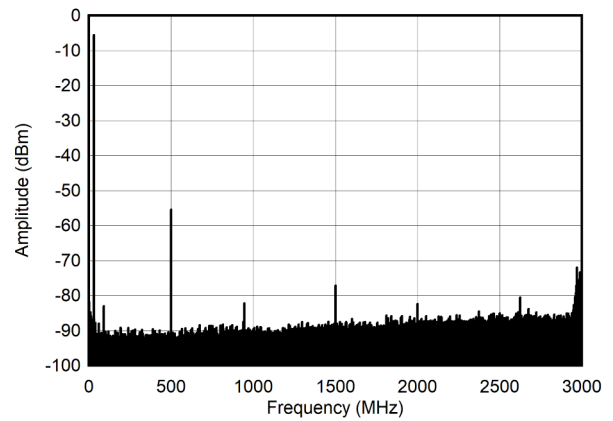
Figure 5-223. Single Tone Spectrum at 30 MHz and -12 dBFS (Nyquist)
