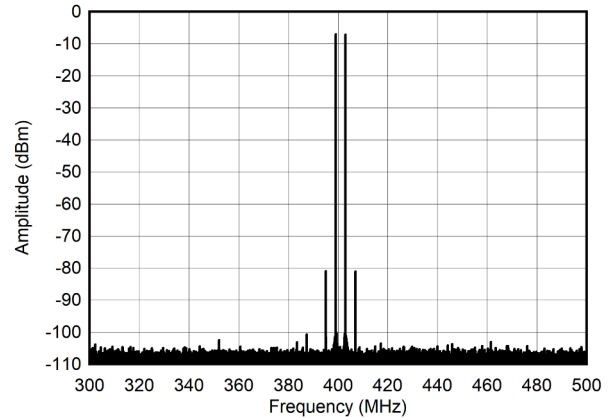
Figure 5-261. Dual Tone Spectrum at 400 MHz and -13 dBFS ( \pm 100 MHz)
