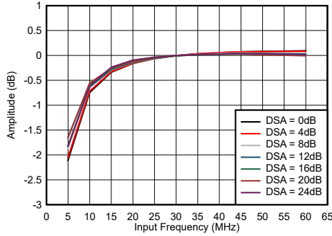
Figure 5-1. RX In-Band Gain Flatness, f_{\text{IN}} = 30\text{ MHz}
