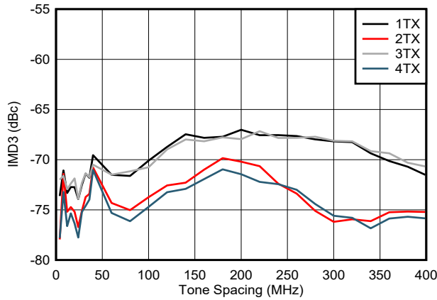
External clock mode, non-interleave mode
