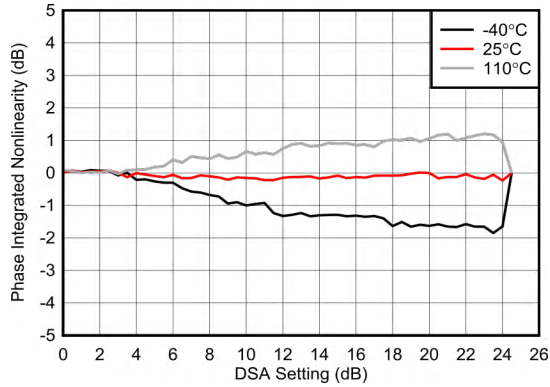
Figure 6-210. RX Calibrated Integrated Phase Error at 6.851GHz
