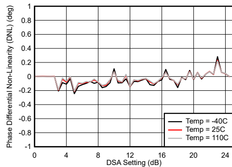
Figure 6-6. RX Uncalibrated Differential Phase Error vs DSA Setting at 30 MHz Differential Phase Error = \text{Phase}_{IN}(\text{DSA Setting} - 1) - \text{Phase}_{IN}(\text{DSA Setting})
