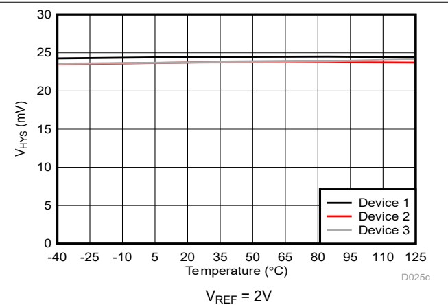
Figure 5-23. Cmp0 Trip Threshold Hysteresis vs Temperature
