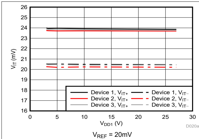
Figure 5-6. Cmp0 Trip Threshold vs Supply Voltage
