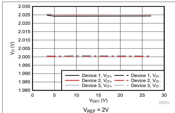
Figure 5-18. Cmp0 Trip Threshold vs Supply Voltage
