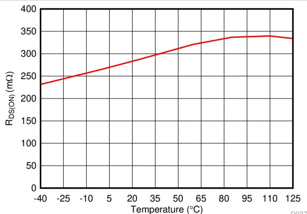
Figure 8-13. R DS(ON) of Low Side MOSFET vs Temperature
