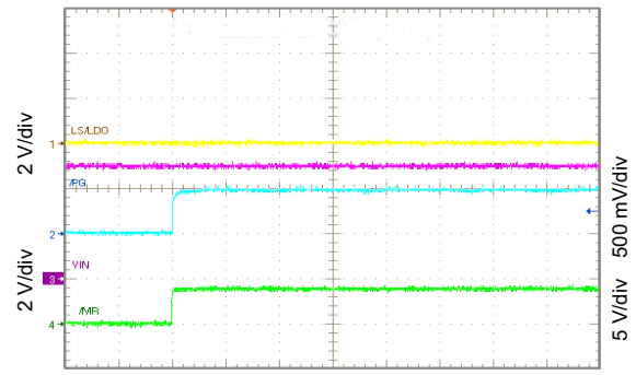
Time 400 μs/div Figure 10-60. PG Functions as Shifted MR Output
