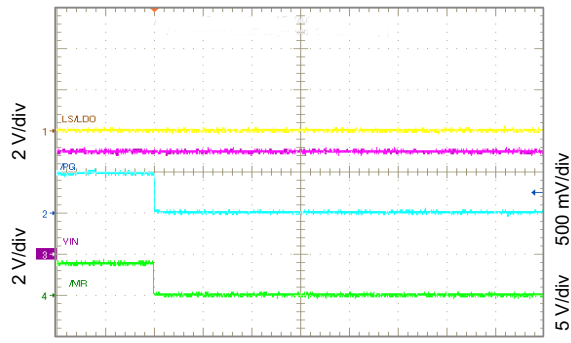
Time 400 μs/div Figure 10-59. PG Functions as Shifted MR Output
