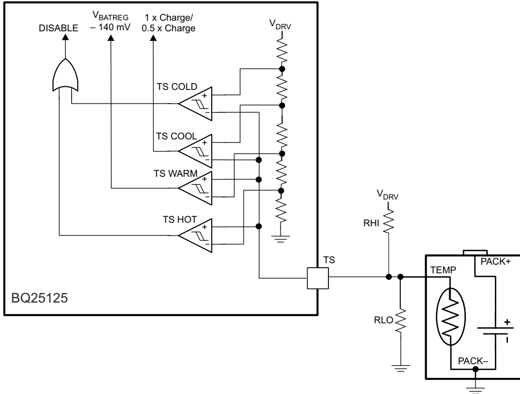
Figure 9-4. TS Circuit
