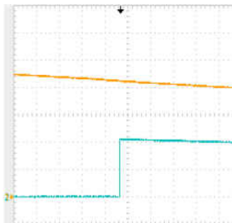
Orange Line (Channel 1) = Decrease Voltage on BAT Pin Turquoise Line (Channel 2) = COUT Gate Drive Output COUT goes from low to high when OVP Recovery = OVP Set Threshold - 100 mV
