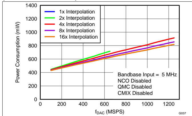
Figure 37. Power Consumption vs f_{DAC} Over Interpolation
