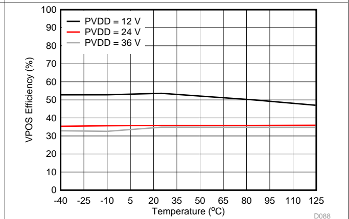
Figure 89. VOUT VPOS Efficiency vs Temperature
