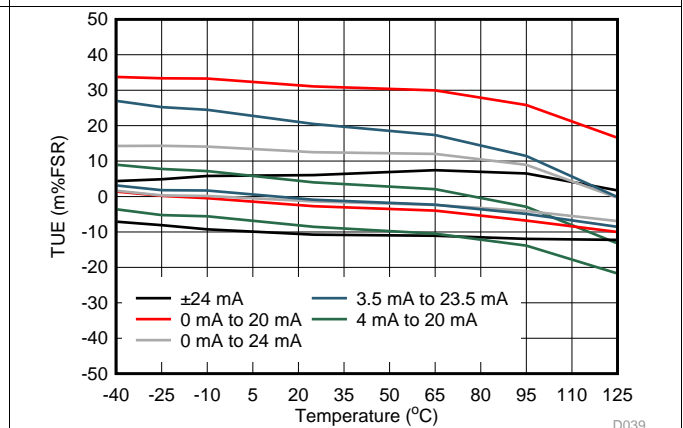
Figure 43. IOUT TUE vs Temperature
