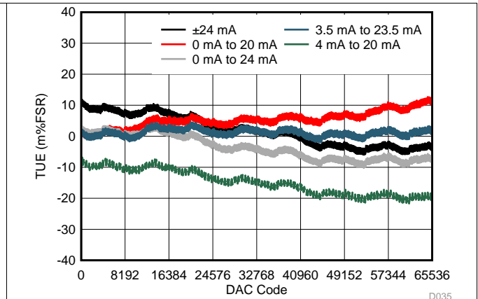
Figure 39. IOUT TUE vs Code (DC/DC Enabled)
