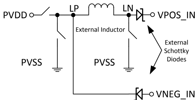
Figure 99. Buck-Boost Converter
