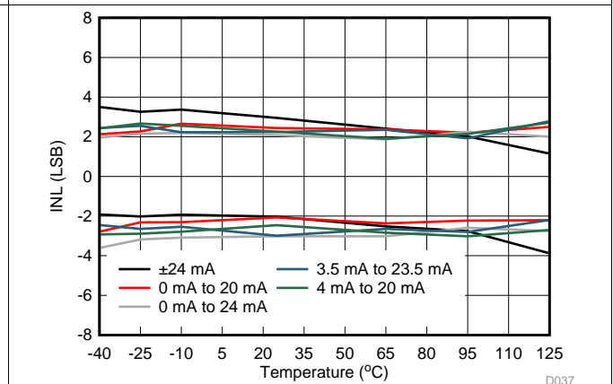
Figure 41. IOUT INL vs Temperature
