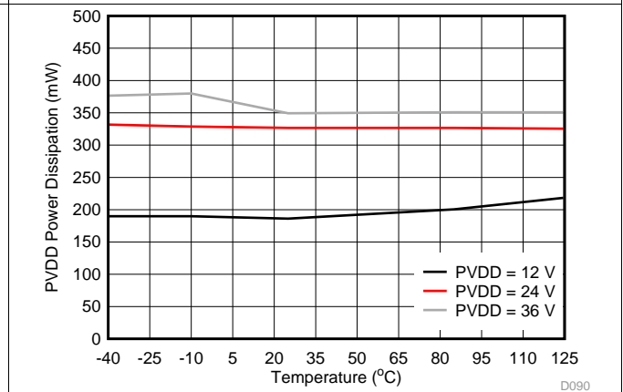
Figure 91. VOUT Power Dissipation vs Temperature
