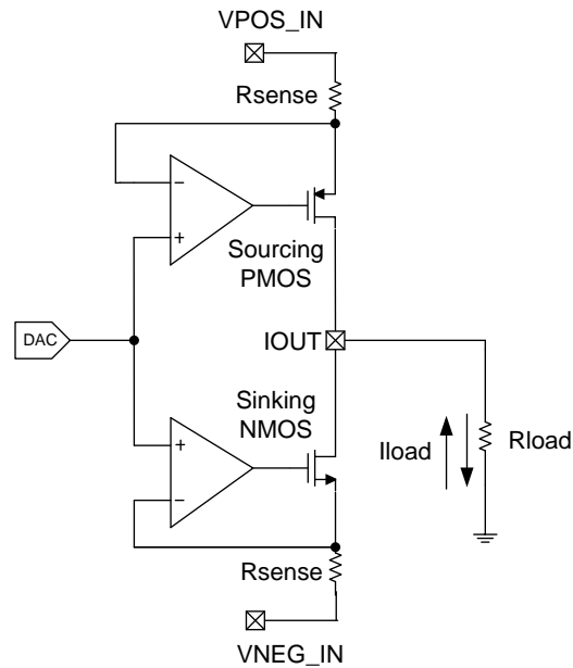
Figure 97. Current Output
