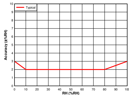
RH Accuracy ( T_A = 30^\circ\text{C} )
