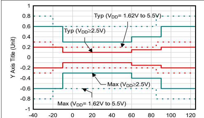
Figure 6-3. T_A Accuracy vs T_A Set Point
