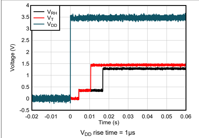
Figure 6-13. Start-up Response
