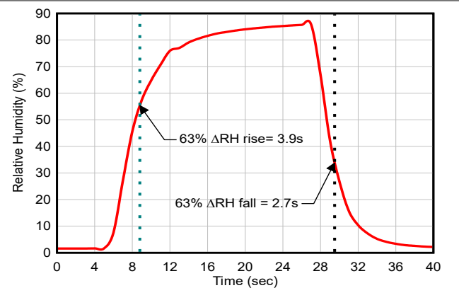
Figure 6-4. Relative Humidity Response Time
