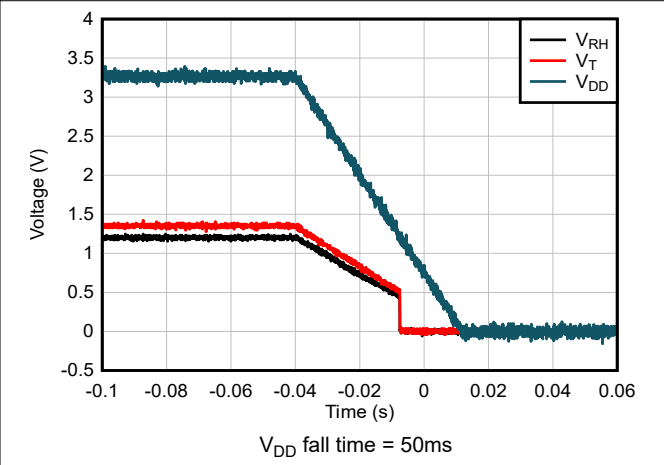
Figure 6-16. Power-down Response
