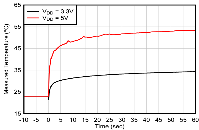
Figure 7-15. Heater Induced Temperature Increase on a Rigid PCB (1.575mm FR4)
