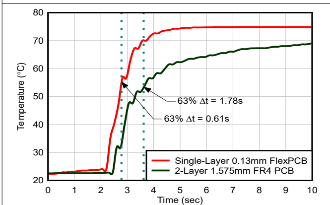
Figure 6-5. Thermal Response Time (Stirred Liquid)
