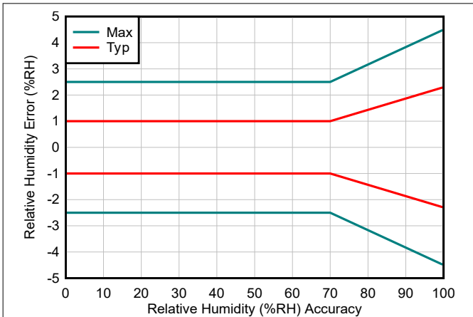
Figure 6-1. RH Accuracy vs RH Set Point ( V_{DD} = 1.62\text{V}-5.5\text{V} )
