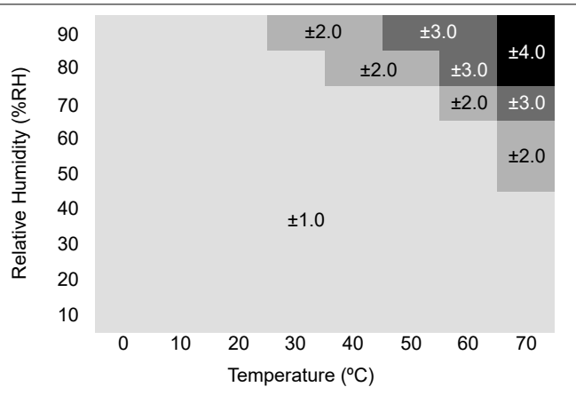
Figure 6-2. RH Typical Accuracy vs T_A Set Point
