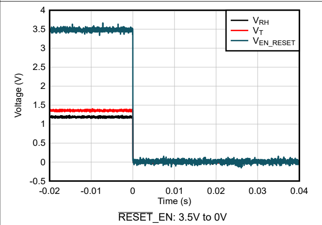
Figure 6-18. Disable Response
