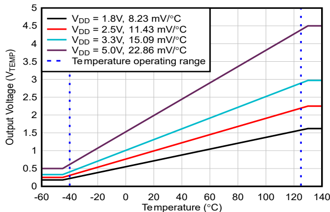
Figure 7-12. Temperature Sensor Output ( V_{\text{TEMP}} ) vs Temperature
