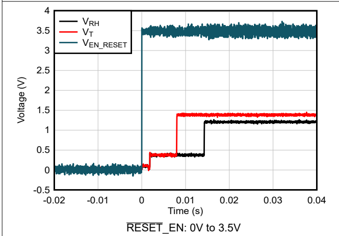
Figure 6-17. Enable Response
