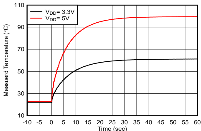
Figure 7-16. Heater Induced Temperature Increase on a FlexPCB (0.13mm Flex)
