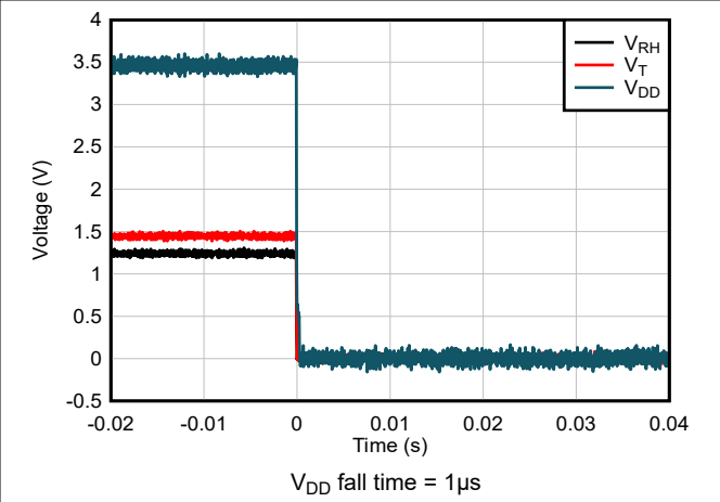
Figure 6-14. Power-down Response
