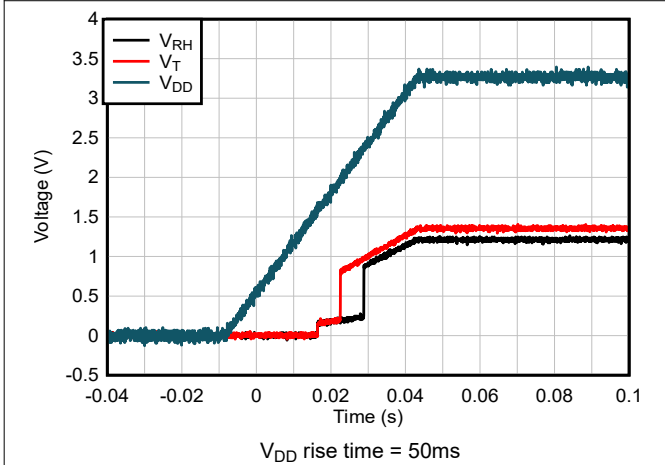
Figure 6-15. Start-up Response
