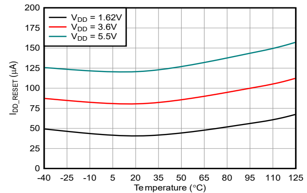
Figure 6-11. Disable Mode Current vs Temperature
