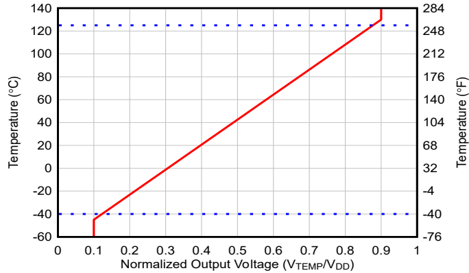
Figure 7-11. HDC3120-Q1 Temperature Output Profile
