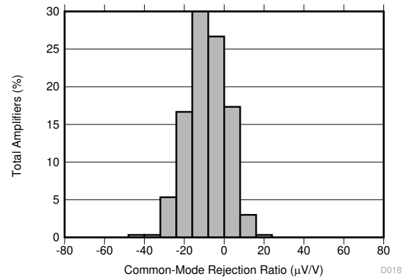
Figure 7-16. Typical CMRR Distribution
