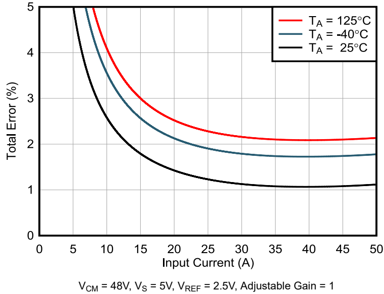
Figure 7-2. INA790B Total Error vs Input Current
