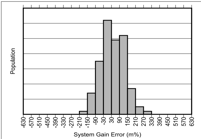
Figure 5-7. INA790B Gain Error Production Distribution
