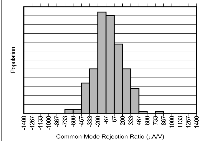
Figure 5-3. INA790B Common-Mode Rejection Production Distribution
