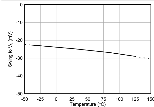
Figure 5-17. Output Voltage Swing High vs Temperature
