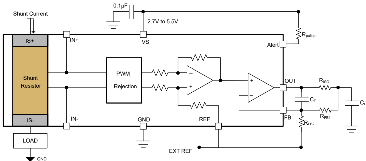
Figure 7-5. INA790x With RISO-Dual-Feedback
