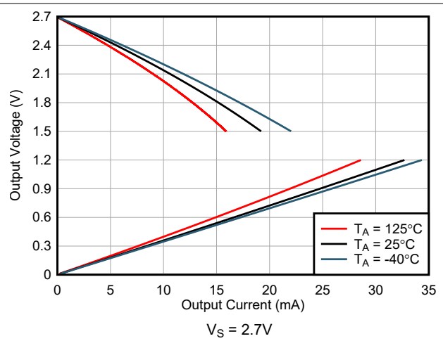
Figure 5-14. Output Voltage Swing vs Output Current
