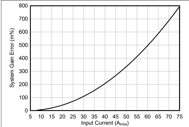
Figure 5-9. INA790B System Gain Error vs Input Current
