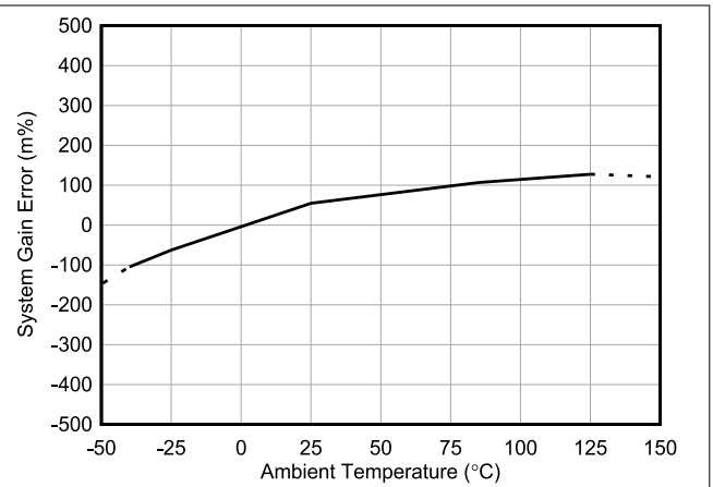
Figure 5-8. INA790B Gain Error vs Temperature
