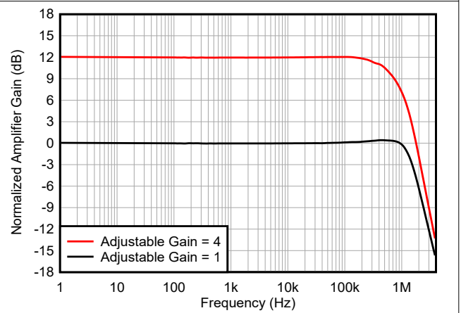
Figure 5-10. Current Sense Amplifier Gain vs Frequency
