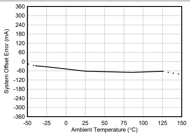
Figure 5-2. INA790B Input Offset Current vs Temperature
