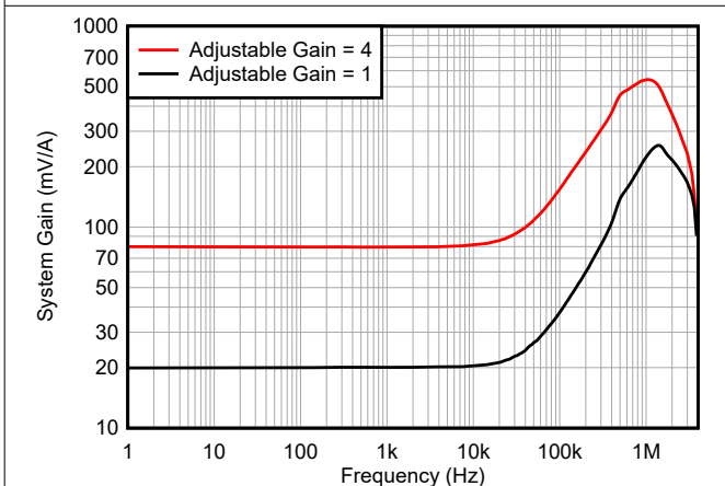
Figure 5-11. System Gain vs Frequency
