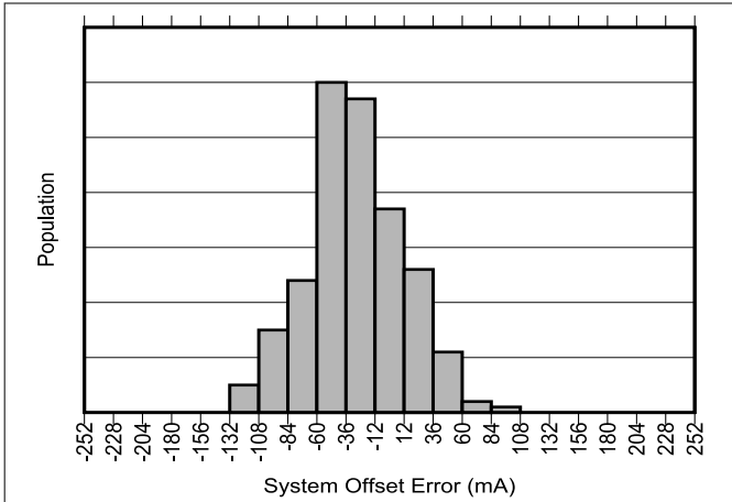
Figure 5-1. INA790B Input Offset Current Production Distribution
