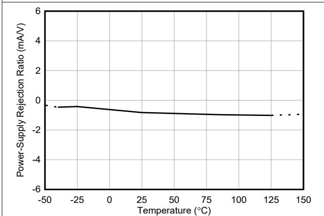
Figure 5-5. Power-Supply Rejection Ratio vs Temperature
