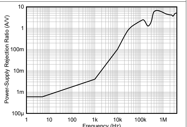
Figure 5-12. Power-Supply Rejection Ratio vs Frequency
