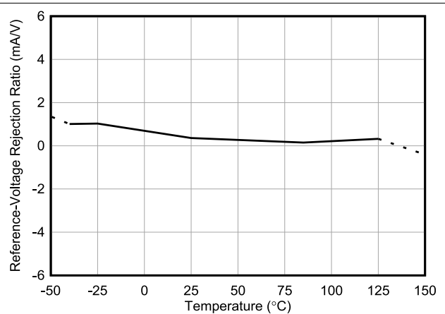
Figure 5-6. Reference Voltage Rejection Ratio vs Temperature
