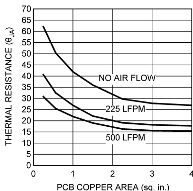
Figure 32. Thermal Resistance vs PCB Area (4 Layer Board)
