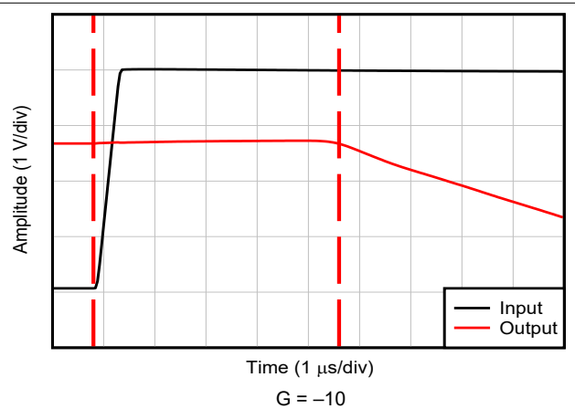
Figure 5-24. Overload Recovery (Positive Rail)
