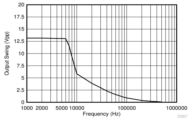
Figure 5-40. Maximum Output Swing vs. Frequency (VCC = 15 V)
