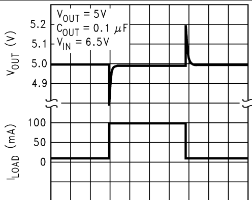
50 \mu\text{s}/\text{Div} Figure 20. Load Transient Response
