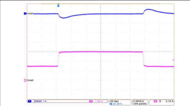
V_{OUT} = 5\text{ V} F_{SW} = 2100\text{ kHz} FPWM mode I_{OUT} = 1.5\text{ A to } 3\text{ A to } 0\text{ A} V_{IN} = 13.5\text{ V} T_R = T_F = 6\text{ }\mu\text{s}
