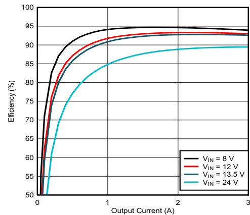
Figure 9-11. LM61430-Q1 Efficiency
