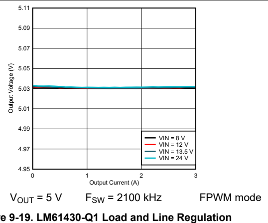
Figure 9-19. LM61430-Q1 Load and Line Regulation
