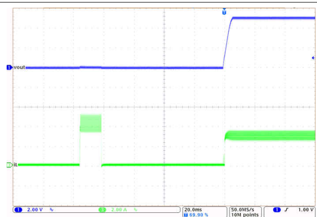
Figure 9-35. LM61430-Q1 Short Circuit Recovery
