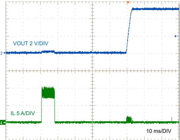
Figure 7-19. Short-Circuit Recovery
