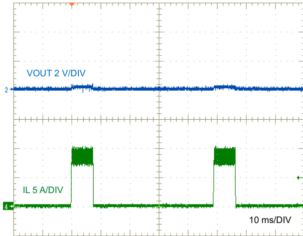
Figure 8-9. LM644x0-Q1 Short-Circuit Hiccup
