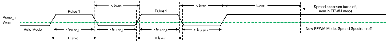
Figure 7-9. Spread Spectrum Disabled in Transition from AUTO Mode to FPWM Mode
