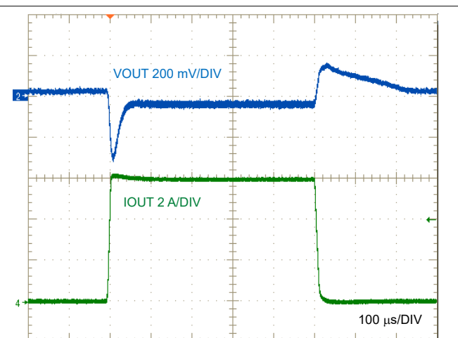
Figure 8-8. LM644x0-Q1 Load Transient, I_{OUT} = 0A to 6A
