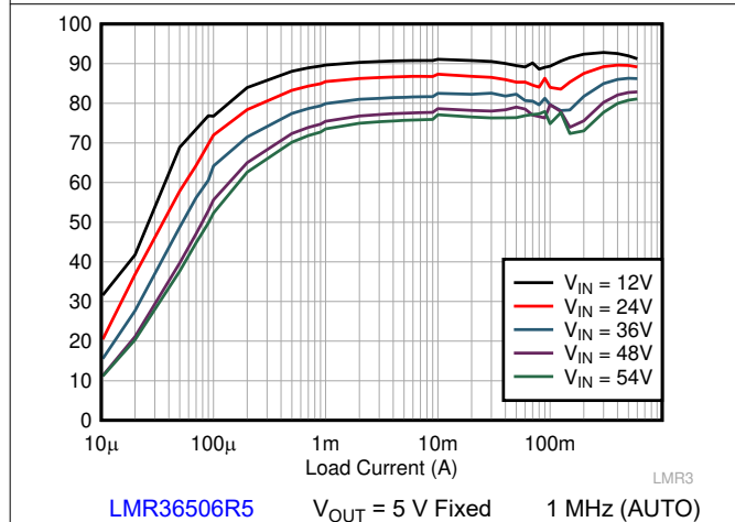
Figure 9-8. Efficiency
