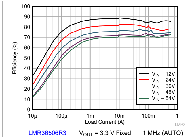
Figure 9-4. Efficiency
