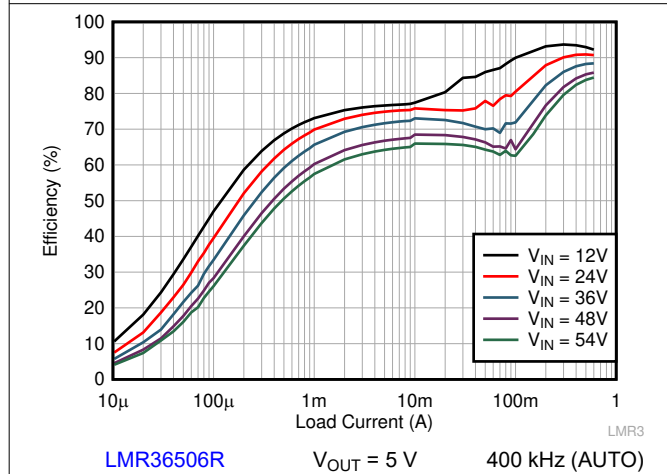
Figure 9-6. Efficiency
