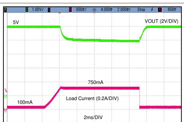
Figure 8-13. Overload Output Recovery (100 mA to 750 mA)
