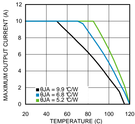
Figure 31. Thermal Derating
