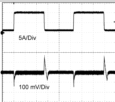
TIME (500 \mu\text{s/Div} ) 12 V_{IN} , 1.2 V_{OUT} , 1- to 10-A Step
