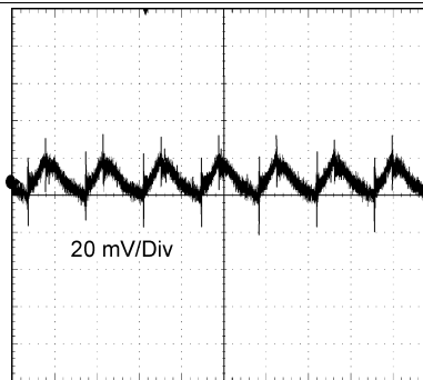
Figure 34. Output Ripple
