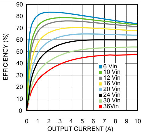
Figure 13. Efficiency 1-V Output at 25°C
