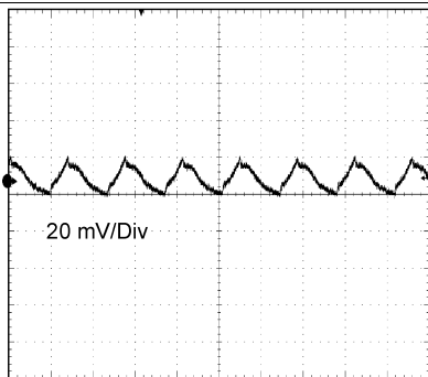
Figure 33. Output Ripple
