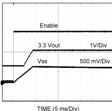
Figure 45. Prebiased Start-Up
