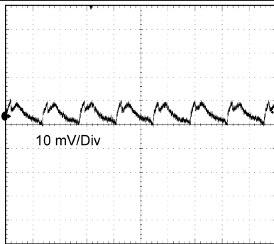
TIME (2 \mu\text{s/Div} ) 12 V_{IN} , 1.2 V_{OUT} at Full Load, BW = 20 MHz
