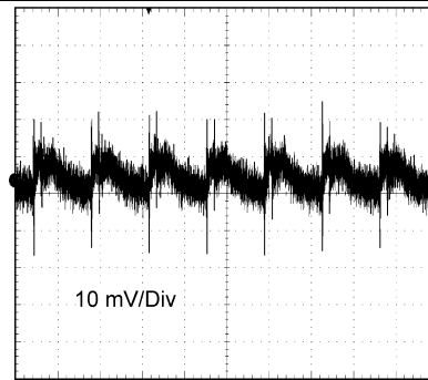
TIME (2 \mu\text{s/Div} ) 12 V_{IN} , 1.2 V_{OUT} at Full Load, BW = 250 MHz
