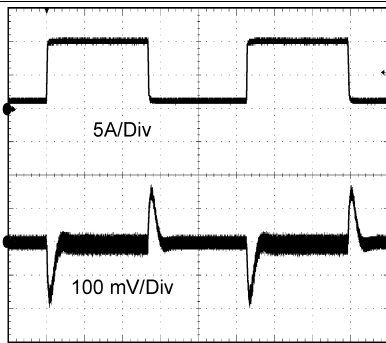
TIME (500 \mu\text{s/Div} ) 12 V_{IN} , 5 V_{OUT} , 1- to 10-A Step
