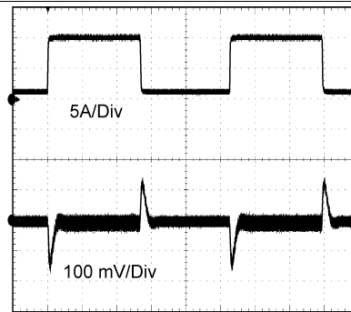
TIME (500 \mu\text{s/Div} ) 12 V_{IN} , 3.3 V_{OUT} , 1- to 10-A Step
