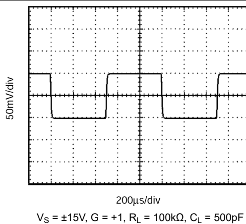
Figure 5-24. OPA251 Small-Signal Step Response
