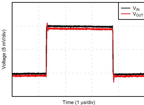
Figure 6-35. Small-Signal Step Response (10-mV Step)
