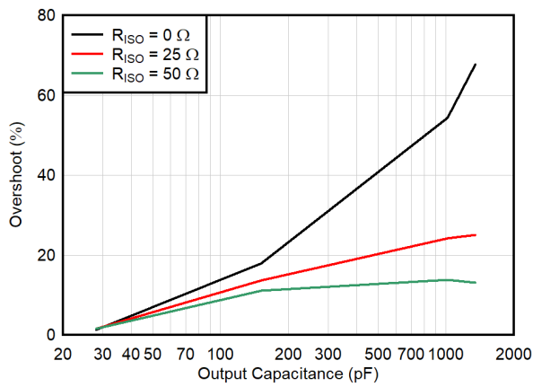
Figure 6-31. Small-Signal Overshoot vs Capacitive Load (10-mV Step)
