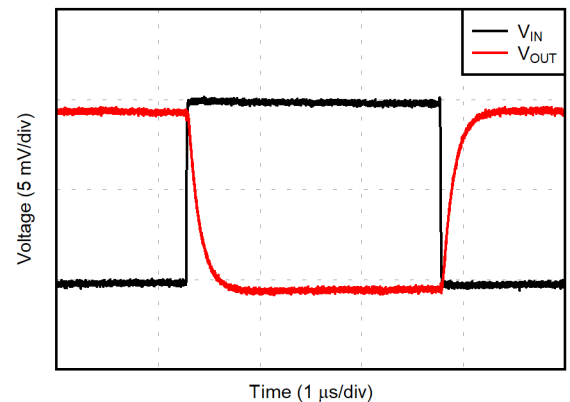
Figure 6-36. Small-Signal Step Response (10-mV Step)
