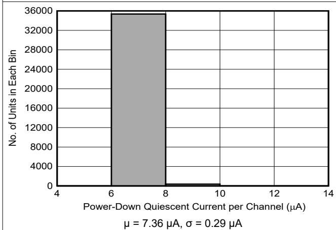
Figure 6-38. Power-Down Quiescent Current Distribution \mu = 7.36\ \mu\text{A} , \sigma = 0.29\ \mu\text{A}
