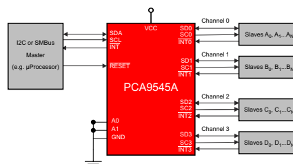
Simplified Application Diagram
