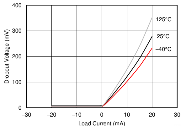
Figure 7-28. Minimum Dropout Voltage vs Load Current
