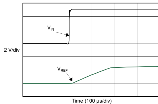
Figure 7-30. Turn-On Settling Time
