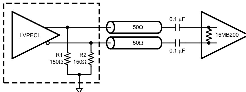
Figure 6. AC Coupled LVPECL to LVDS Interface
