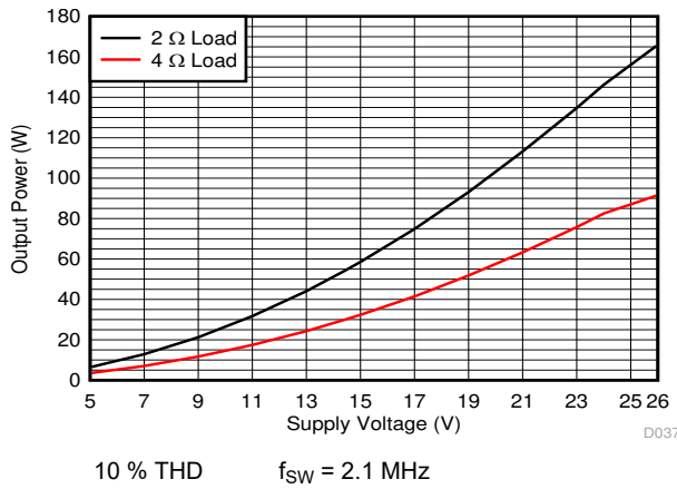
Figure 7-31. PBTLM Output Power vs Voltage
