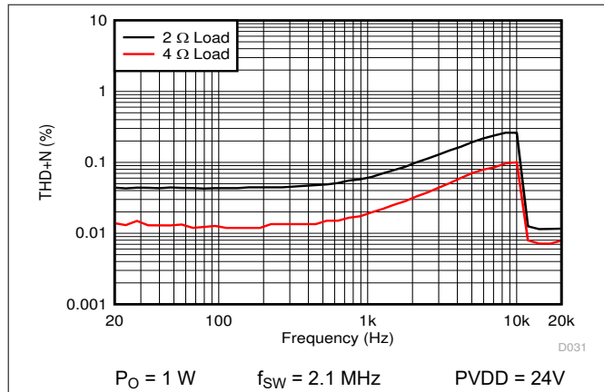
Figure 7-25. PBTL THD+N vs Frequency
