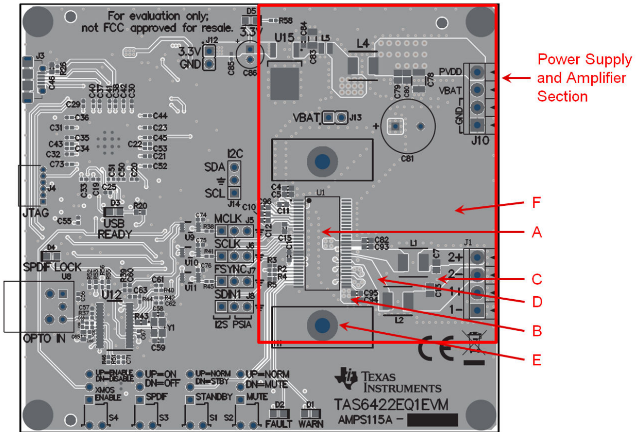
Figure 12-1. EVM Layout
