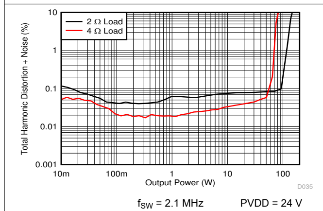
Figure 7-29. PBTL THD+N vs Power
