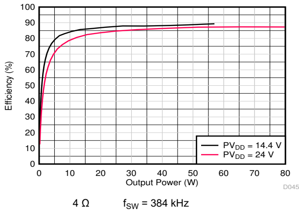
Figure 7-15. Power Efficiency vs Total Output Power
