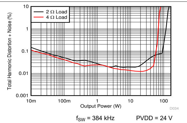
Figure 7-28. PBTL THD+N vs Power
