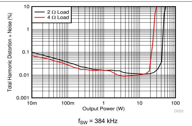
Figure 7-26. PBTL THD+N vs Power
