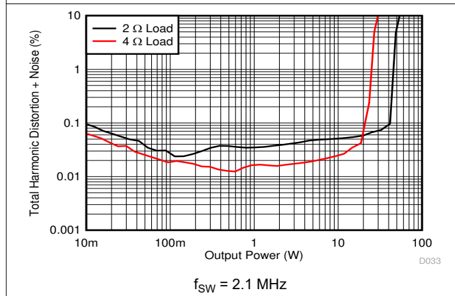
Figure 7-27. PBTL THD+N vs Power
