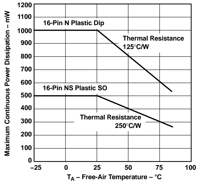
Figure 28. Maximum Continuous Power Dissipation vs Free-Air Temperature
